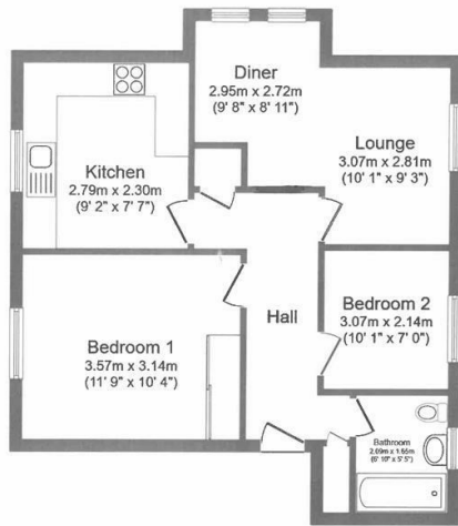
Floor Plan
